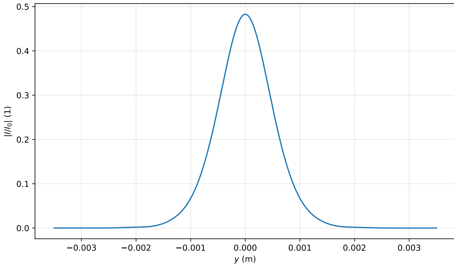
Intensity profile I(x=0, y, z=3.981)/I_0 , P_{in}=0.6P_{cr} , artificial time
